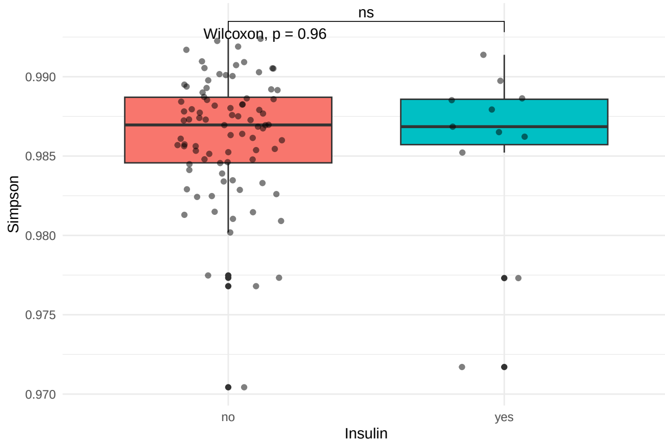
Simpson Diversity by Insulin Use
